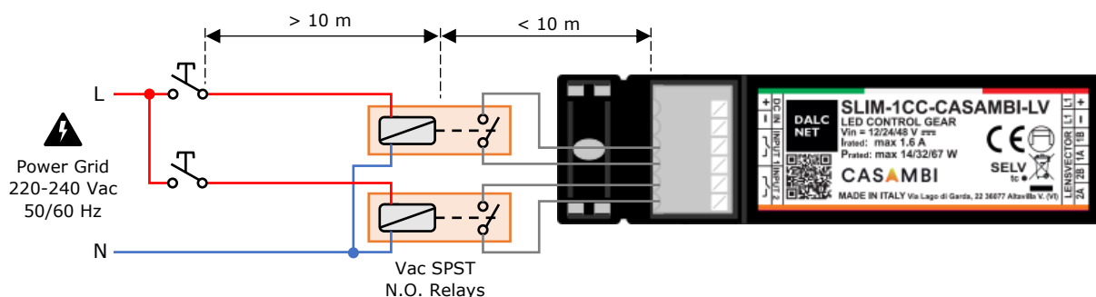
Figure 4: Local Command connection diagram for Long Distances
