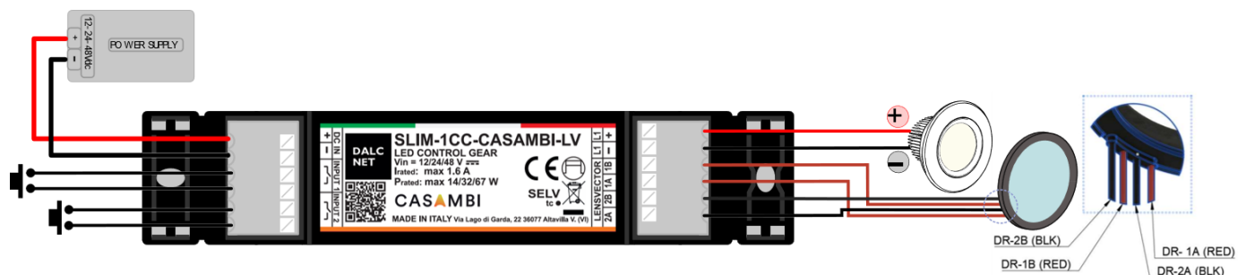
Figure 2: Connection diagram for White or Single-Colour LED load and LensVector® lens
