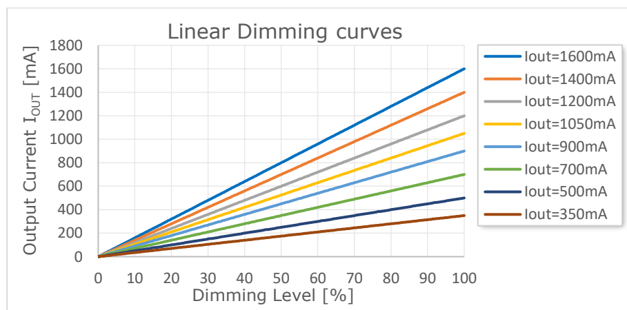
Figure 8: Linear curves according to the Output Current set
